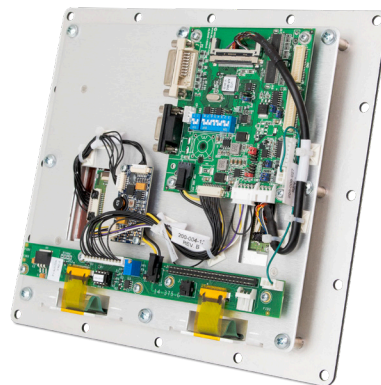
Mil-spec Saber PanelMount Solar 6.5 UPB shown with custom bezel buttons, and lacks a rear enclosure to simplify mounting
